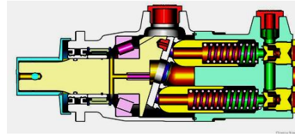
Axial piston pump
